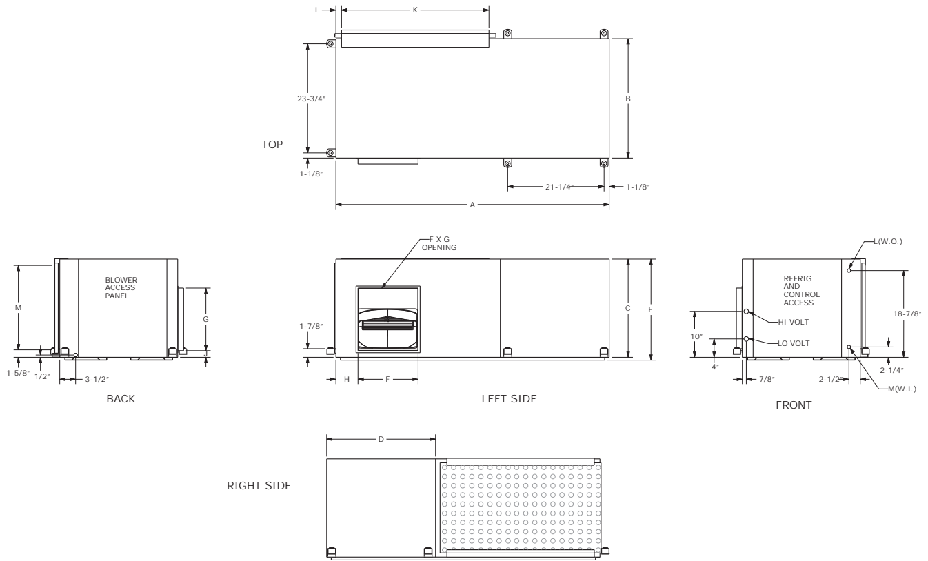
Figure 22. Right return/left supply VSH
