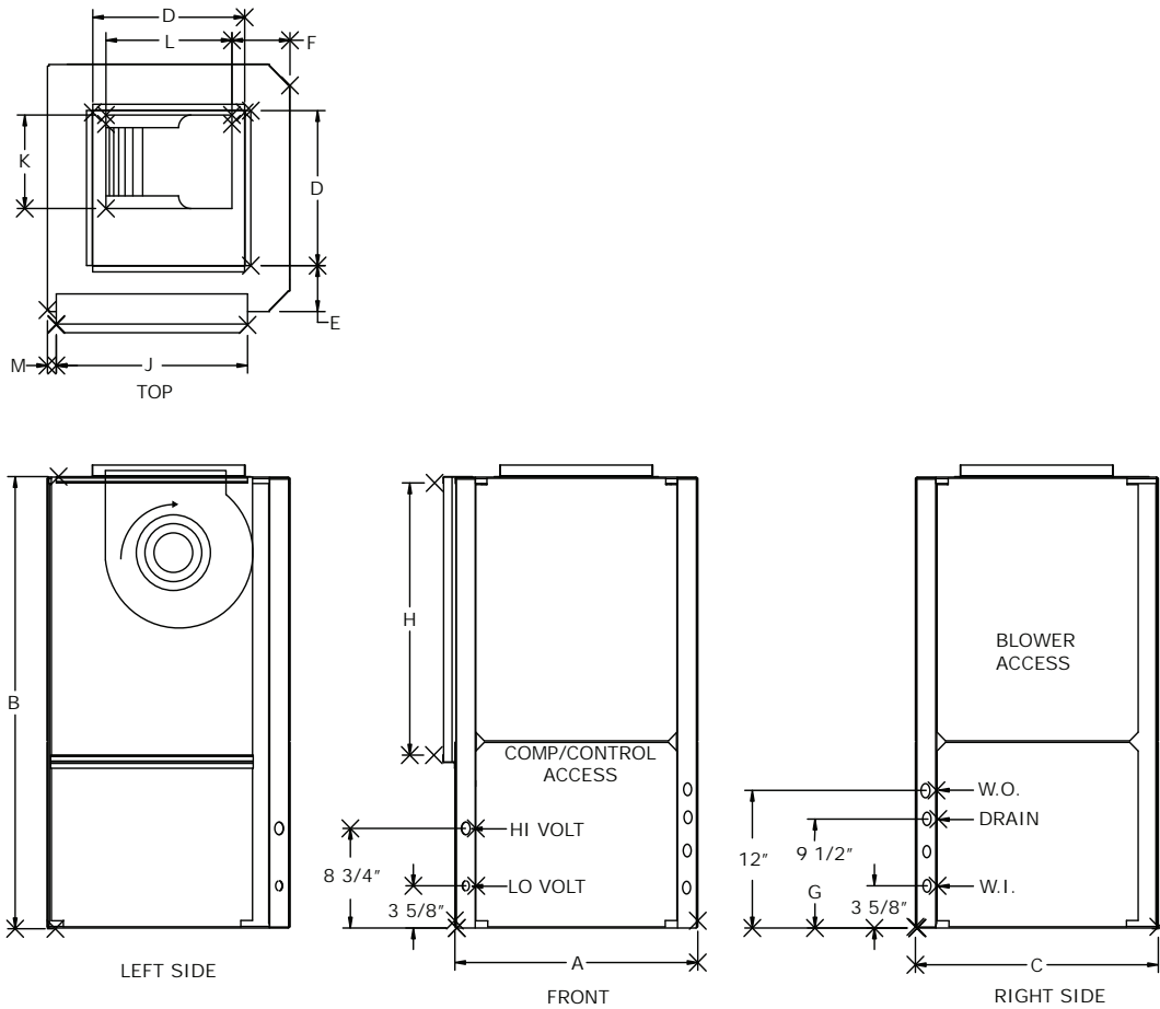
Figure 11. Left return/top supply VSV
