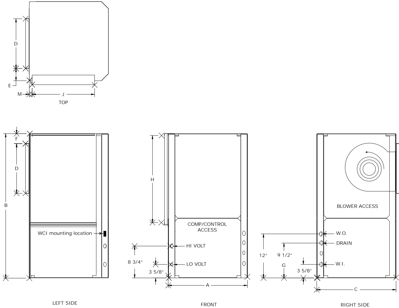
Figure 13. Left return/back supply VSV
