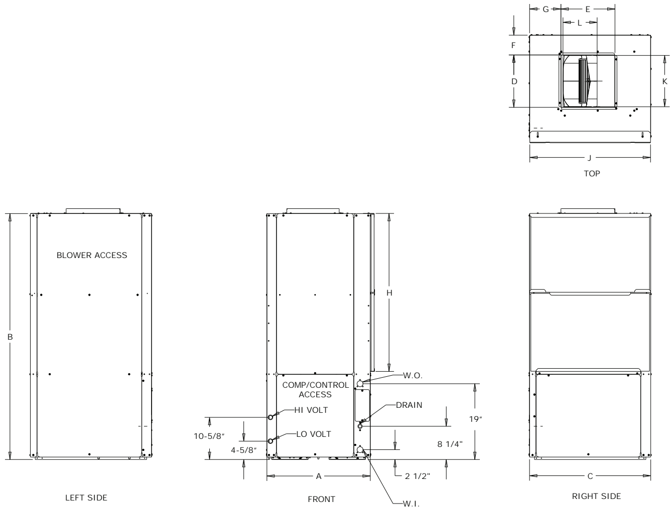
Figure 16. Right return/top supply VSV
