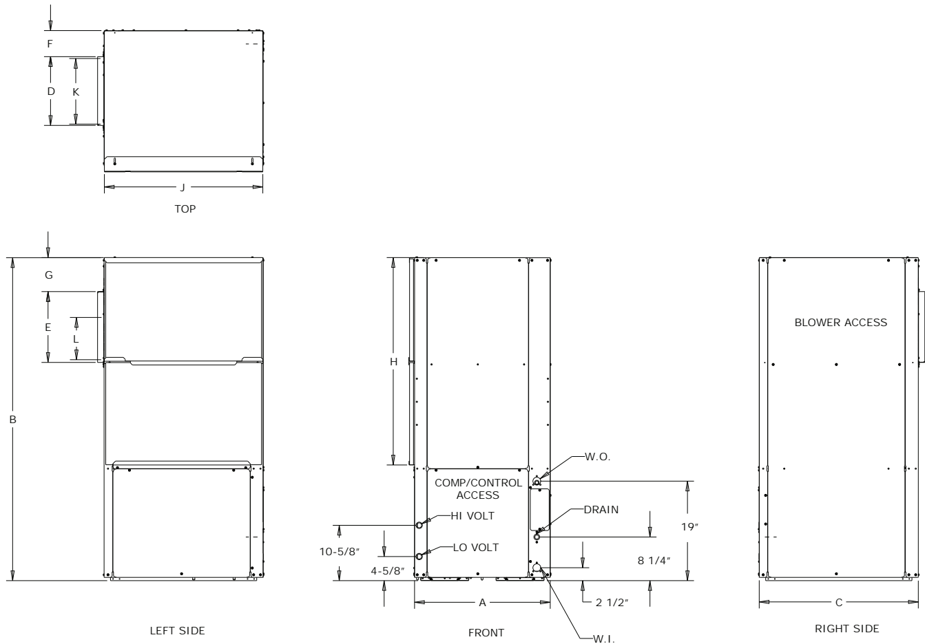
Figure 14. Left return/back supply VSV
