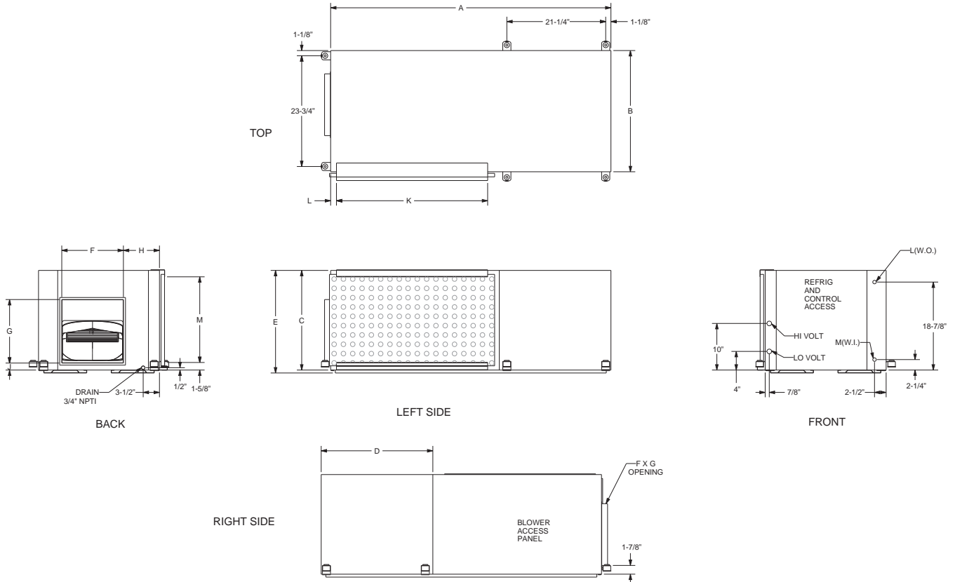
Figure 19. Left return/back supply VSH
