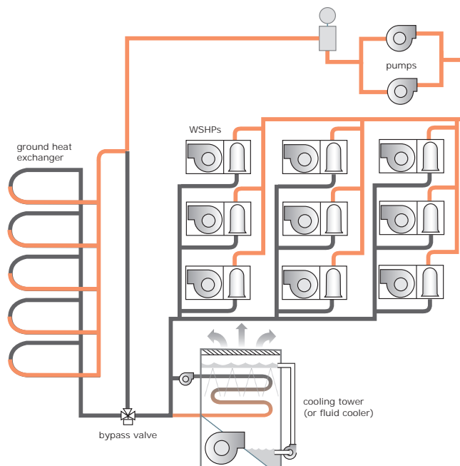
Figure 3. Hybrid system
