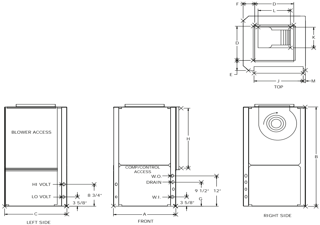
Figure 15. Right return/top supply VSV
