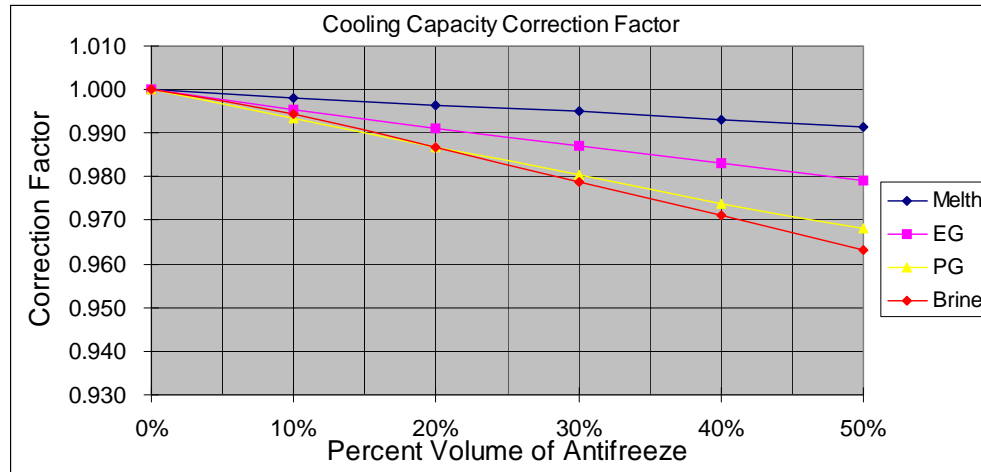
Figure 8. Cooling capacity correction factor
