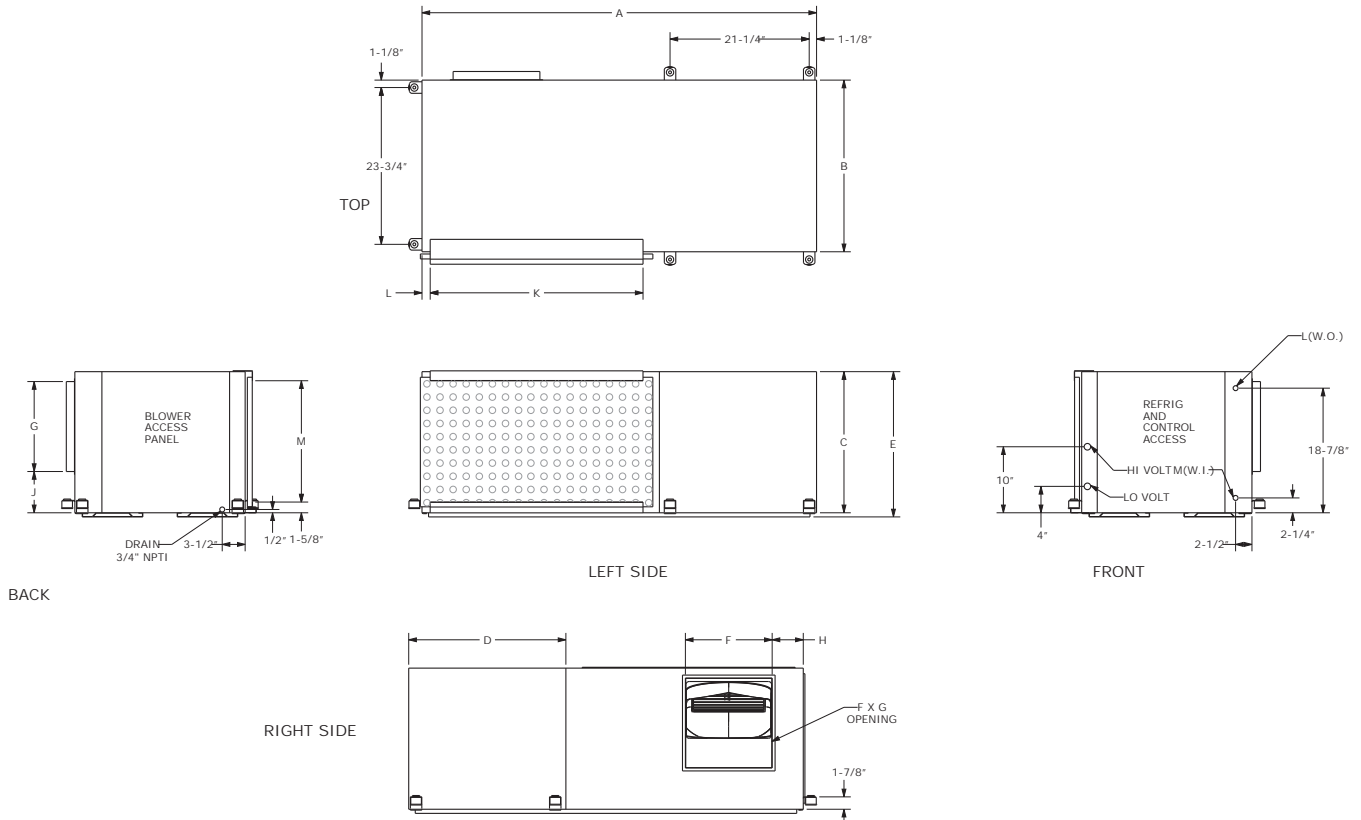
Figure 20. Left return/right supply VSH
