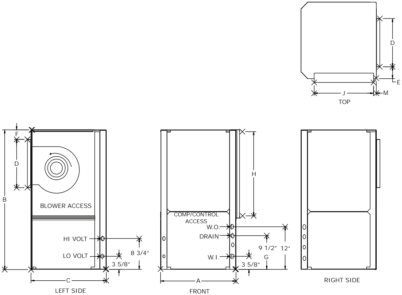
Figure 17. Right return/back supply VSV
