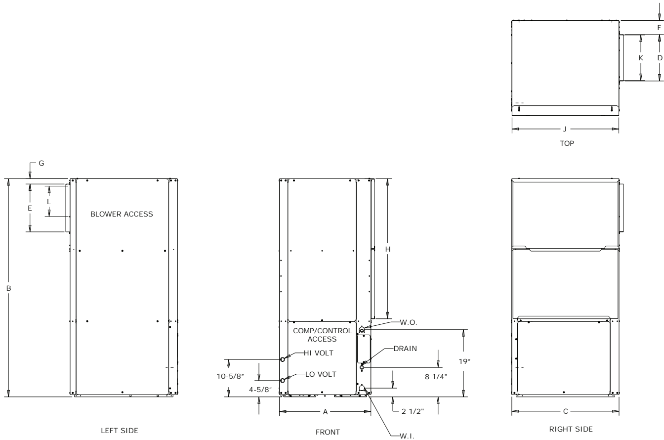
Figure 18. Right return/back supply VSV
