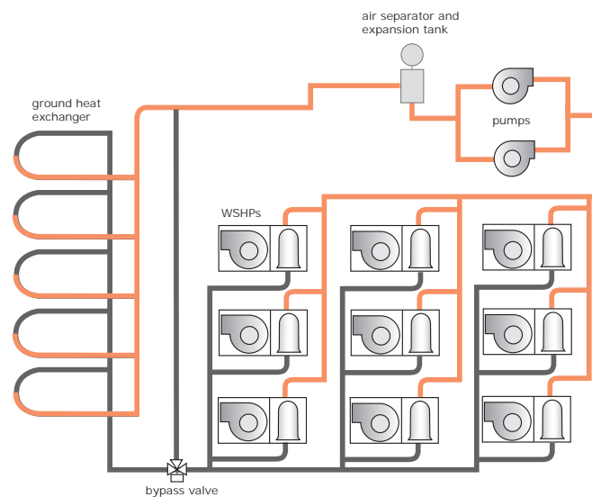
Figure 2. Ground source heat pump system
