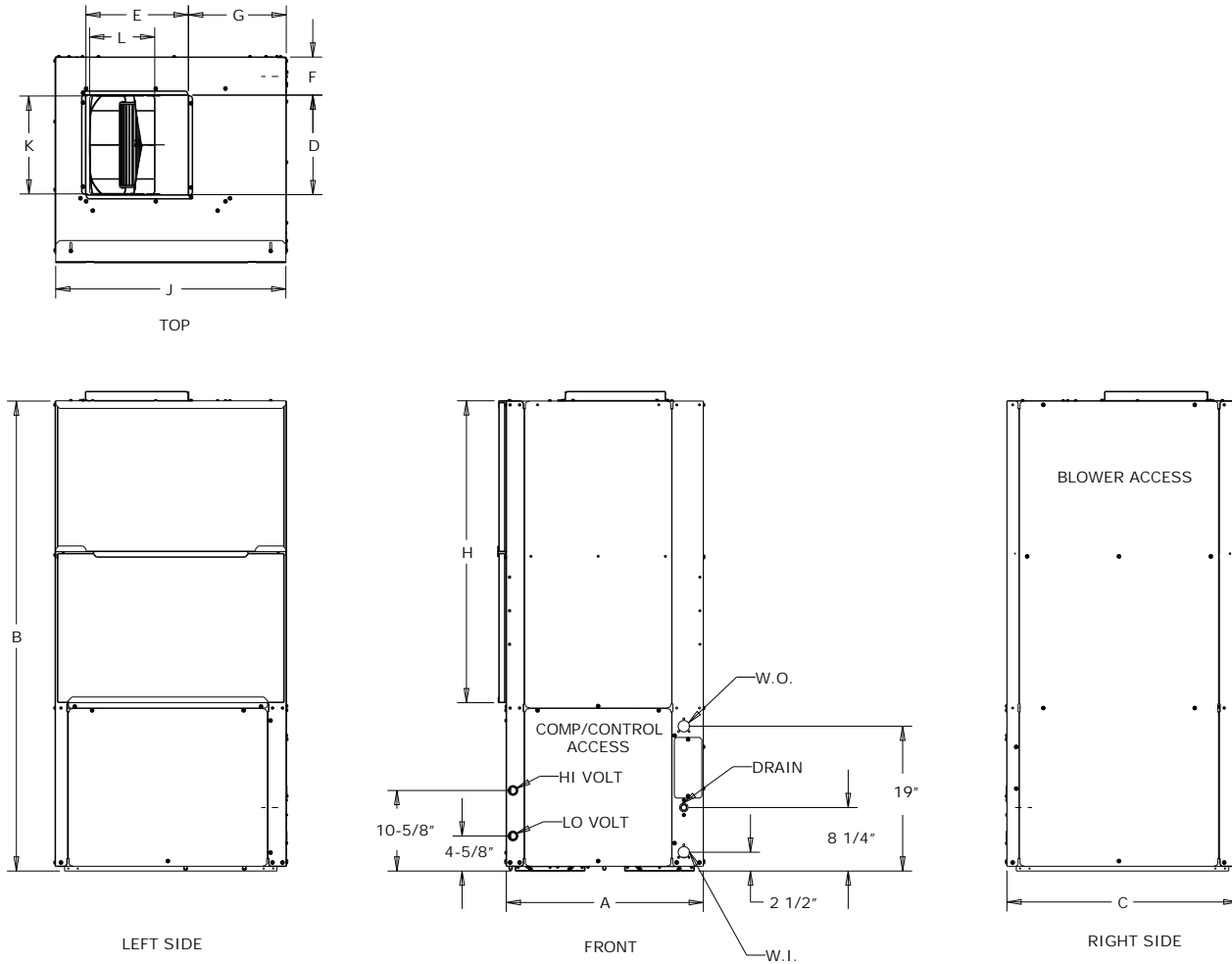
Figure 12. Left return/top supply VSV
