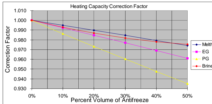
Figure 9. Heating capacity correction factor
