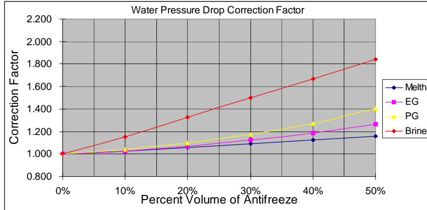
Figure 10. Water pressure drop correction factor
