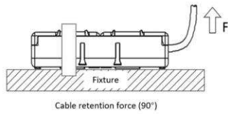
Figure 1 Cable retention force
