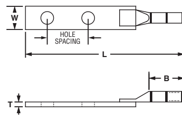
Figure 2: Two Piece Brazed Tongue Construction
