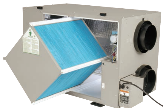
ERV/HRV High-Efficiency Core
