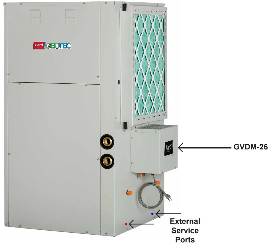
GV Unit with optional GVDM-26 Domestic Hot Water Desuperheater Pump Module (Field-Installed)
